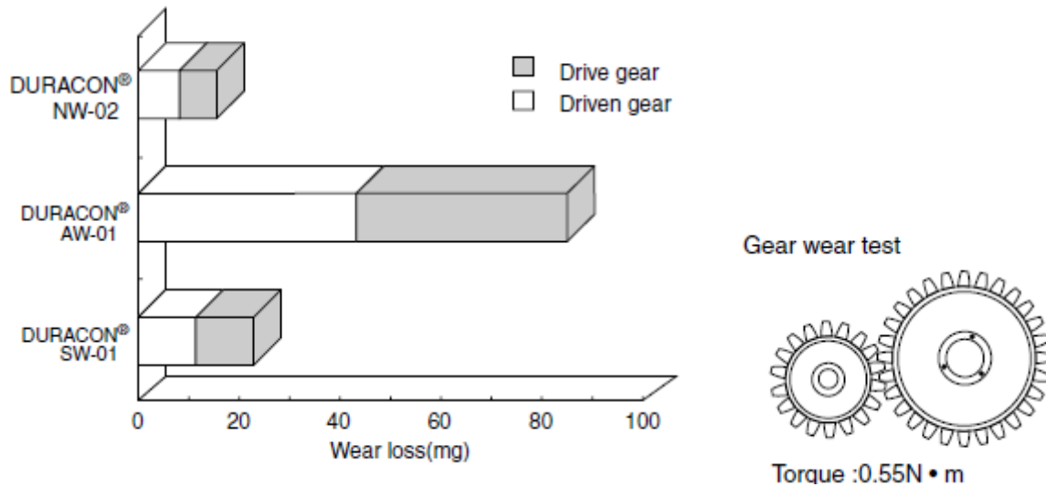
Fig. 1-7 Gear wear characteristics under high load (against the same material)
