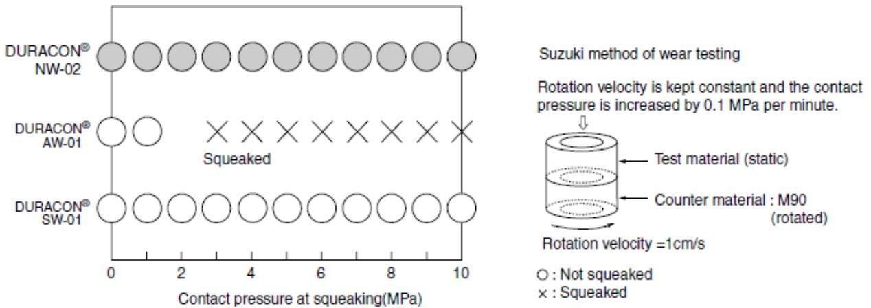
Fig. 2-1 Squeaking noise generation behavior
